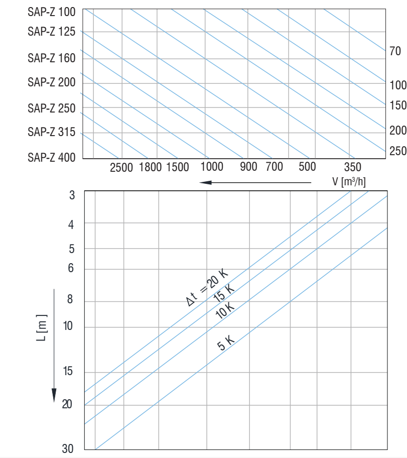
Vertical warm air jet SAP-Z
